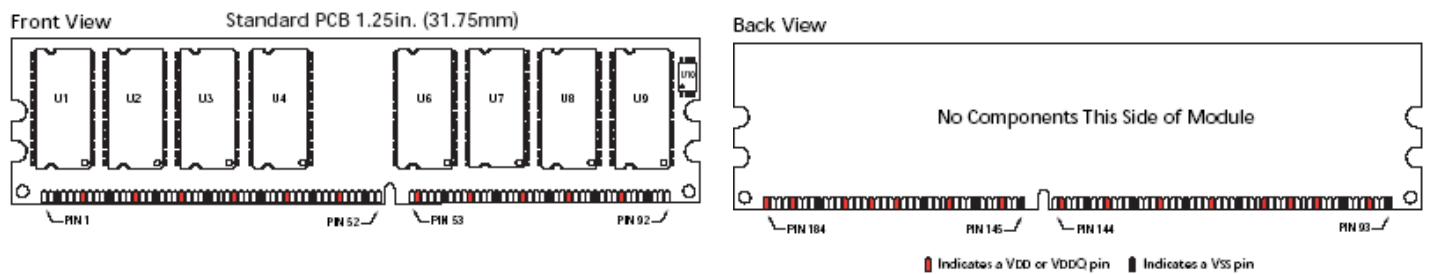
Figure 2: Pin Locations
