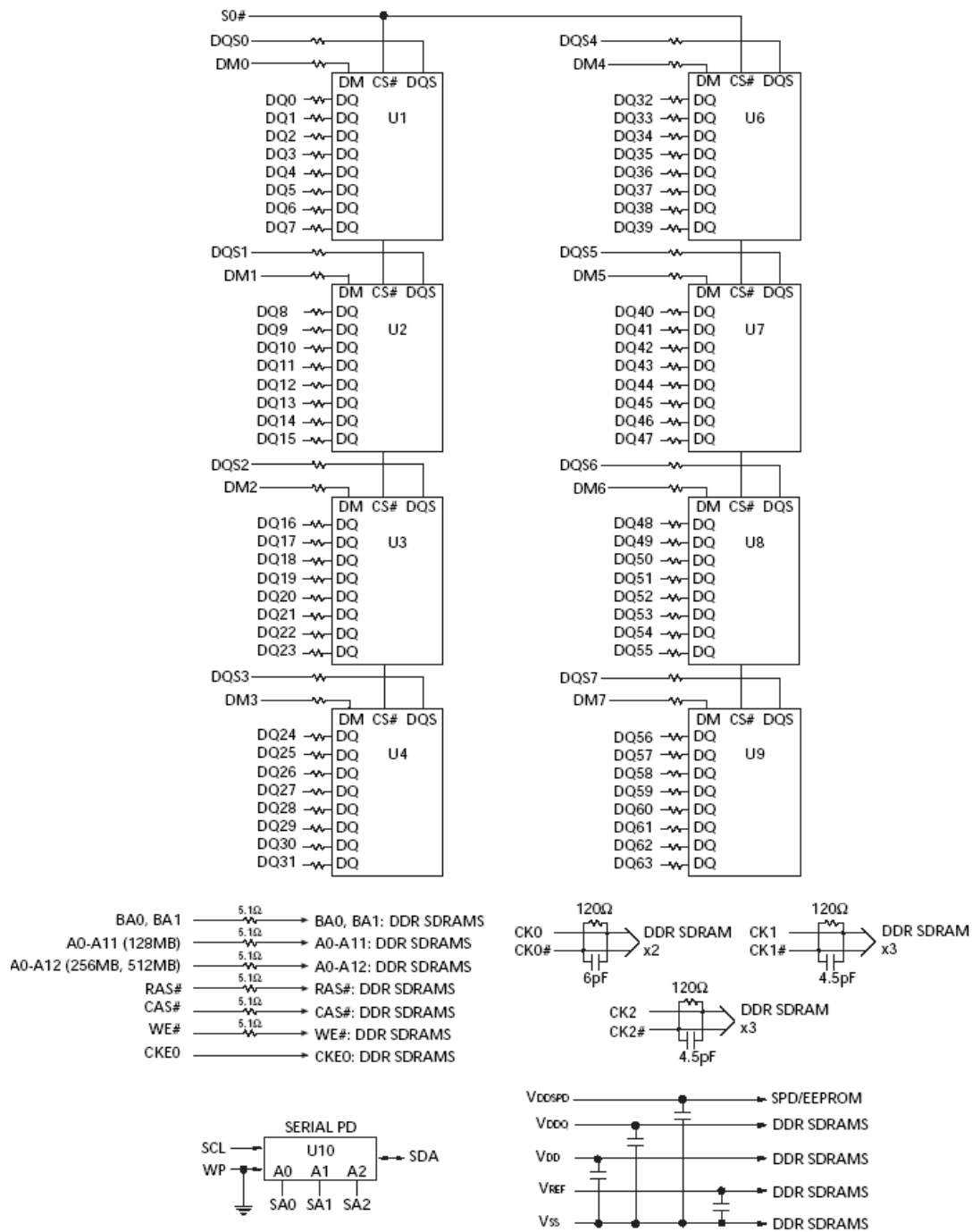
Figure 3: Functional Block Diagram
